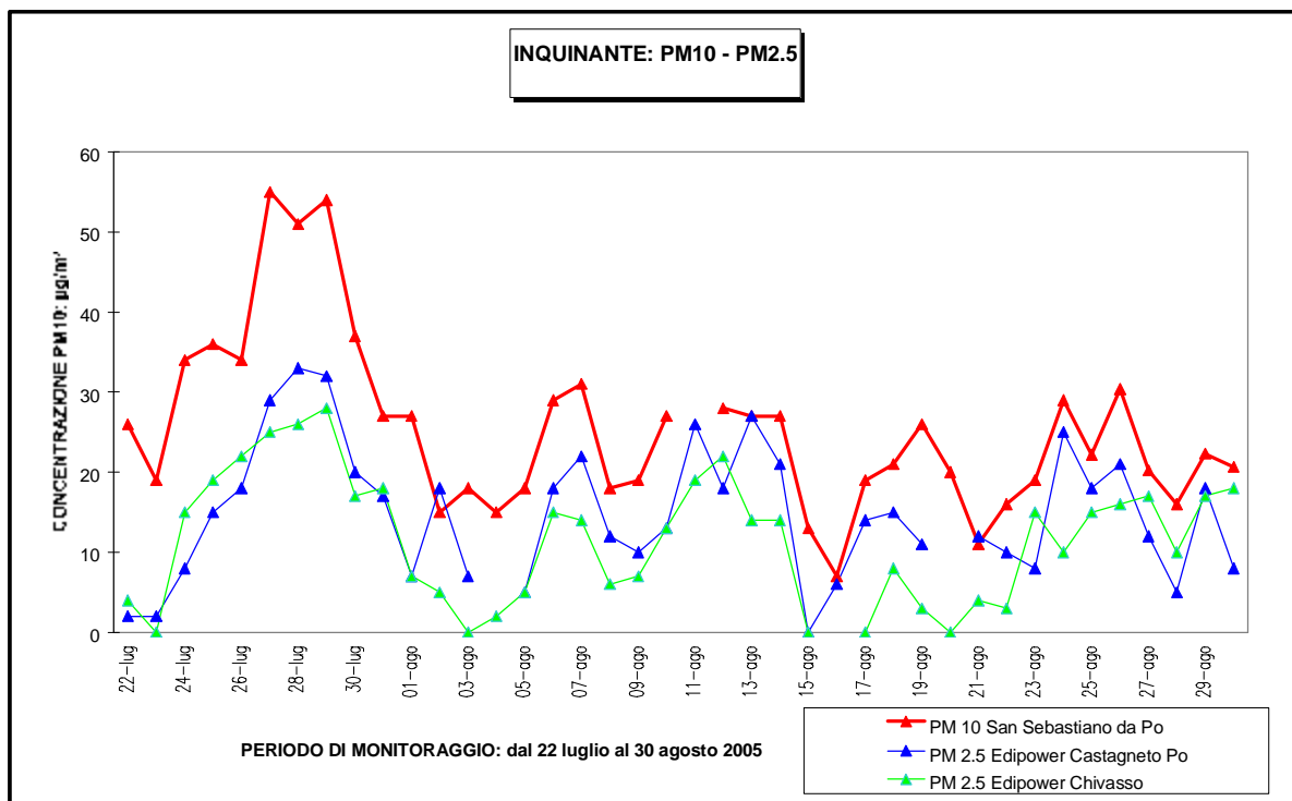
Figura 29: PM 10 / PM 2.5
